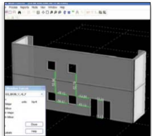
Shear wall forces displayed at any cross section.
